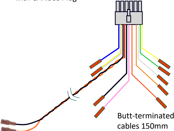
5m twisted pair with red Posi-Taps
